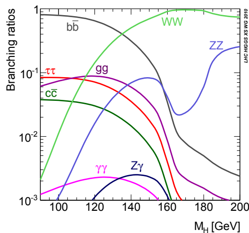
Fig. 1 List of most significant decay channels branch ratio. (Courtesy from CERN website [5]).
