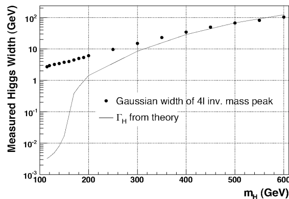
Fig. 2 Total Higgs width. The dots are simulation results from CMS (Physics TDR) for the H \rightarrow ZZ^* \rightarrow 4 leptons final state sub-threshold decay. The solid line is the Standard Model prediction. (Courtesy from Tully’s talk [6]).
